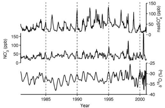
Fig. 2. Profiles of non-sea-salt sulfate ( \text{nssSO}_4^{2-} ), nitrate ( \text{NO}_3^- ) and oxygen isotope ratios ( \delta^{18}\text{O} ) in US ITASE core 2000-1, from 1981 to 2001. Note the distinct rise in sulfate levels beginning in 1991/92, due to the Pinatubo eruption. Dashed lines are for reference and show 1 January of selected years.
