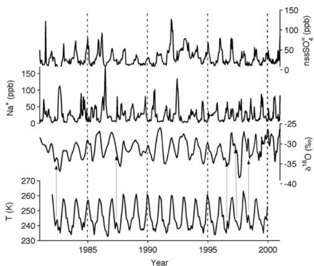
Fig. 4. Same as Figure 3, but for US ITASE core 2001-5, and showing sodium concentrations ( \text{Na}^+ ) in place of nitrate. Arrows show suggested correlations between mid-winter warming events and mid-winter oxygen isotope anomalies.
